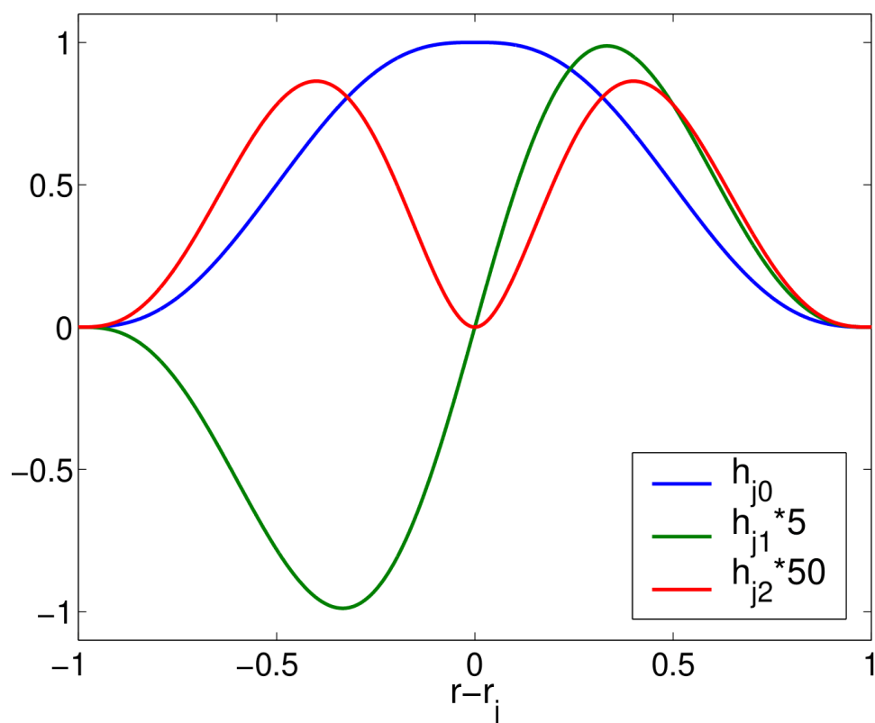
Fig. 29.1: Basis functions h_{j0} , h_{j1} , and h_{j2} are shown. We note that at the left and right extremes, the values and first two derivatives of the functions are zero; while at the center, h_{j0} has a value of 1, h_{j1} has a first derivative of 1, and h_{j2} has a second derivative of 1.
