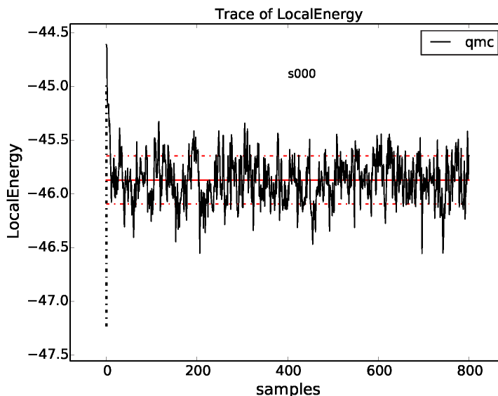
Fig. 12.1: Trace of the VMC local energy for an 8-atom cell of diamond generated with qmca . The x-axis (“samples”) refers to the VMC block index in this case.
