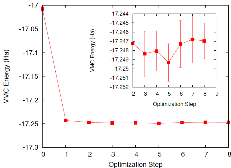
Fig. 21.1: VMC energy as a function of optimization step.
