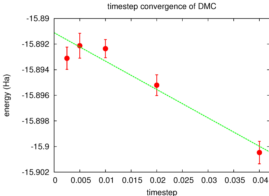
Fig. 20.1: Linear fit to DMC timestep data from PlotTstepConv.pl .
