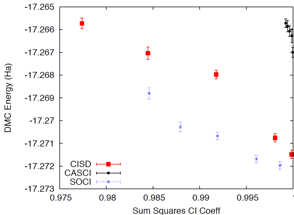
Fig. 21.5: DMC energy as a function of the sum of the square of CI coefficients from CISD.
