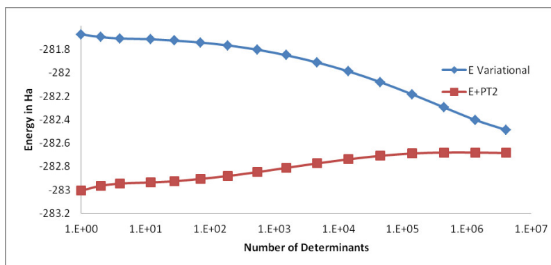
Fig. 15.2: Evolution of the variational energy and the Energy + PT2 as a function of the number of determinants for the C_2O_2H_3N molecule.
