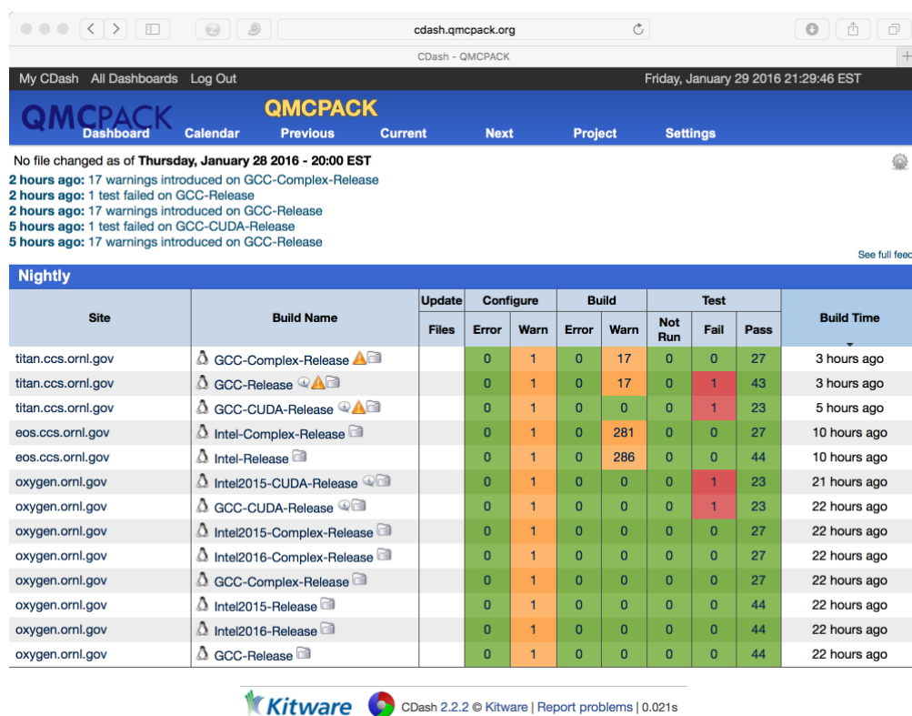
Fig. 4.1: Example test results for QMCPACK showing data for a workstation (Intel, GCC, both CPU and GPU builds) and for two ORNL supercomputers. In this example, four errors were found. This dashboard is accessible at https://cdash.qmcpack.org
